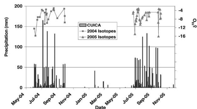
FIGURE 6. (A) Daily precipitation (bars) and volumetric soil moisture (dots) as measured at the Nevado de Colima site from 2001 to 2005 (see Biondi et al., 2005, for details). Percentages indicate the monsoon precipitation (June to October) with respect to the total precipitation for the water year (June to May). Arrows indicate the timing of the isotopic sampling events at the Nevado de Colima study area. (B) Stable isotopic composition of monsoon precipitation events, and precipitation amounts, as collected in Colima City during the monsoon, 2004–2005.
